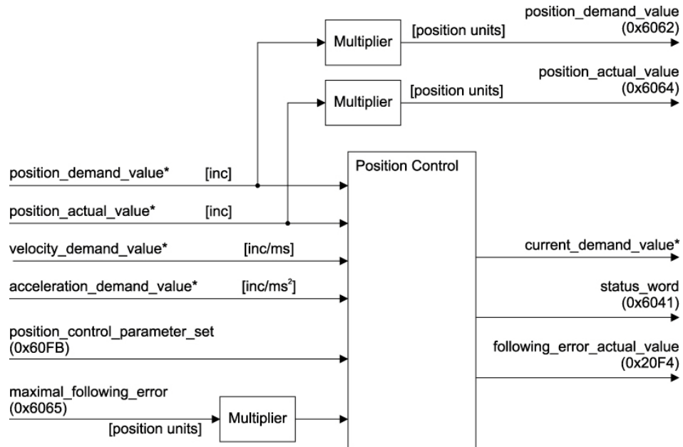
Figure 5-31 Position Control Function – Block Diagram
