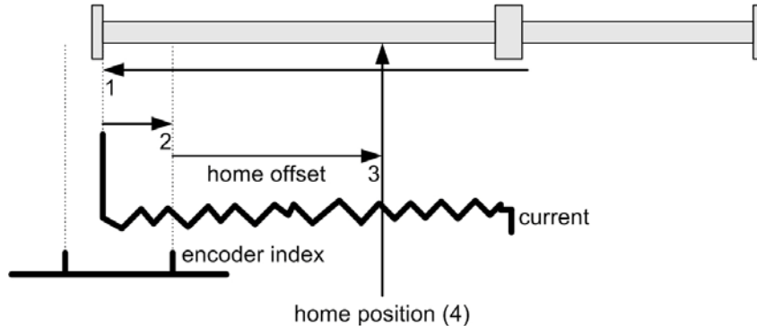
Figure 5-19 Homing Method -2
