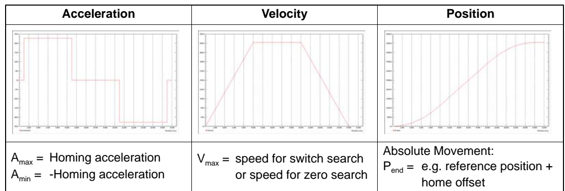
Figure 5-11 Homing Trajectory – Linear Ramp (trapezoidal Profile)
