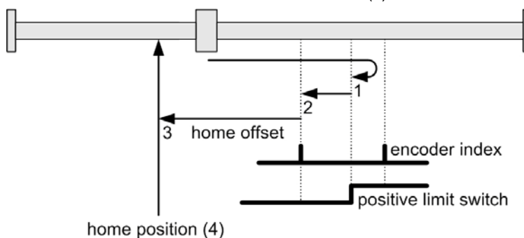
Figure 5-14 Homing Method 2
