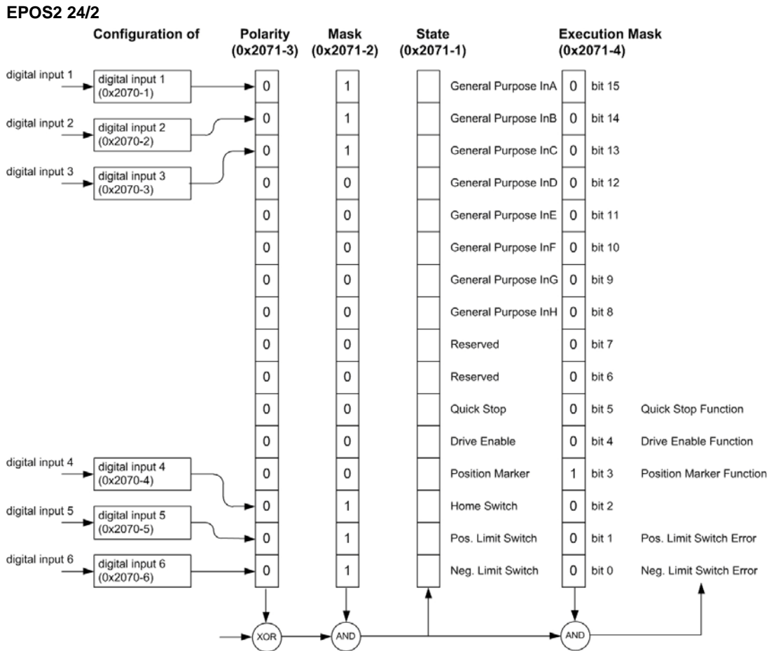
Figure 6-48 Digital Input Functionality – EPOS2 24/2 Overview (Default Configuration)
