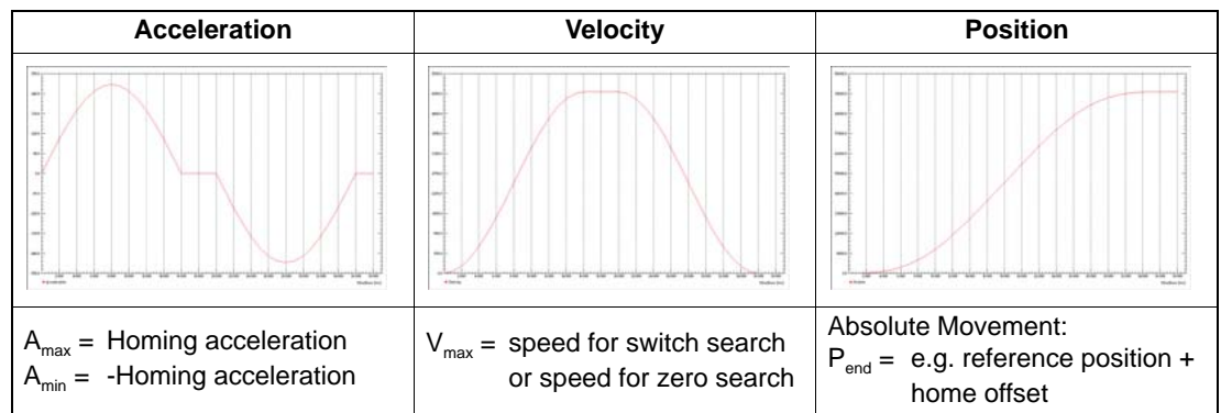
Figure 5-12 Homing Trajectory – Sin² Ramp (sinusoidal Profile)
