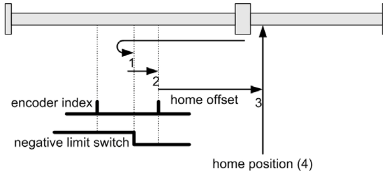
Figure 5-13 Homing Method 1
