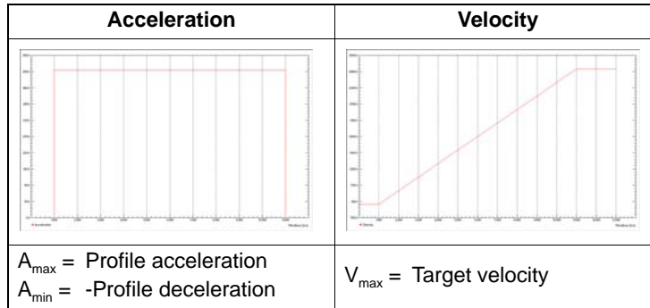
Figure 5-34 Profile Velocity Trajectory – Linear Ramp (trapezoidal Profile)
