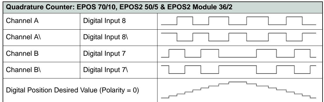
Figure 5-26 Master Encoder Mode – Quadrature Counter 1
