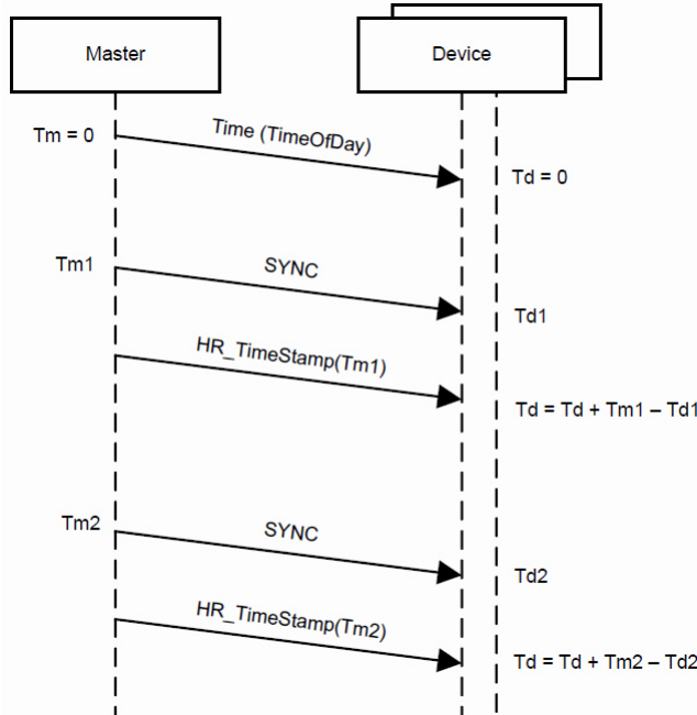
Figure 5-21 Interpolated Position Mode – Clock Synchronization
