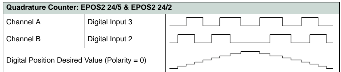
Figure 5-27 Master Encoder Mode – Quadrature Counter 2
