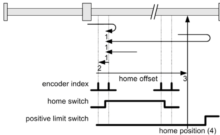
Figure 5-15 Homing Method 7
