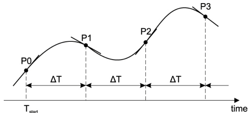
Figure 5-20 Interpolated Position Mode – PVT Principle
