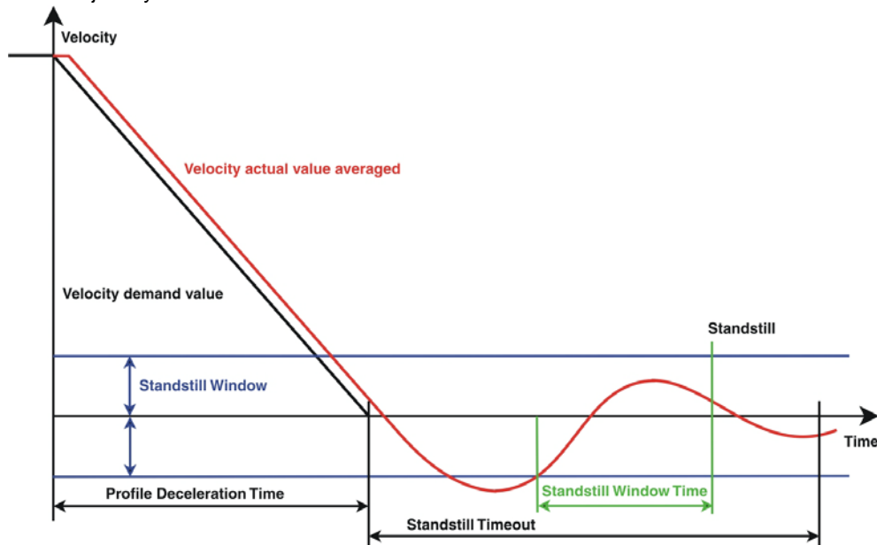
Figure 8-78 Standstill Window
