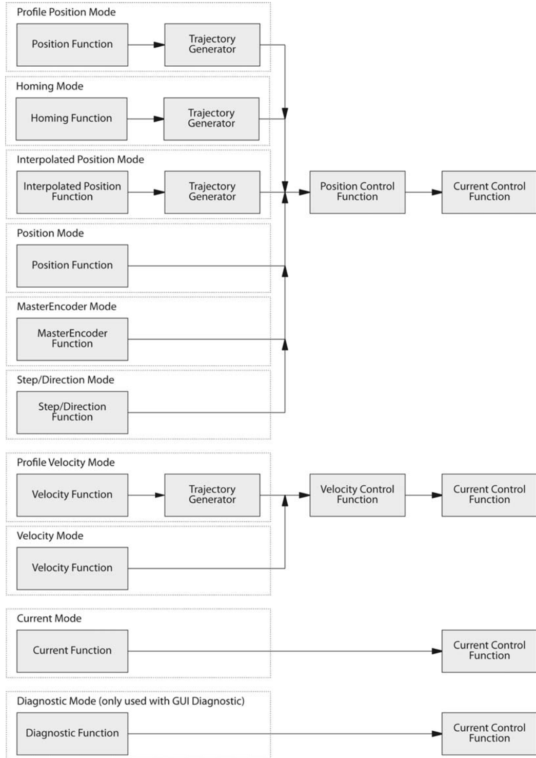
Figure 5-4 Functional Architecture
