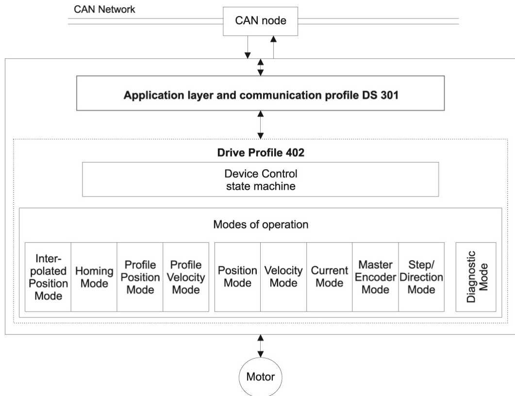
Figure 3-2 Communication Architecture
