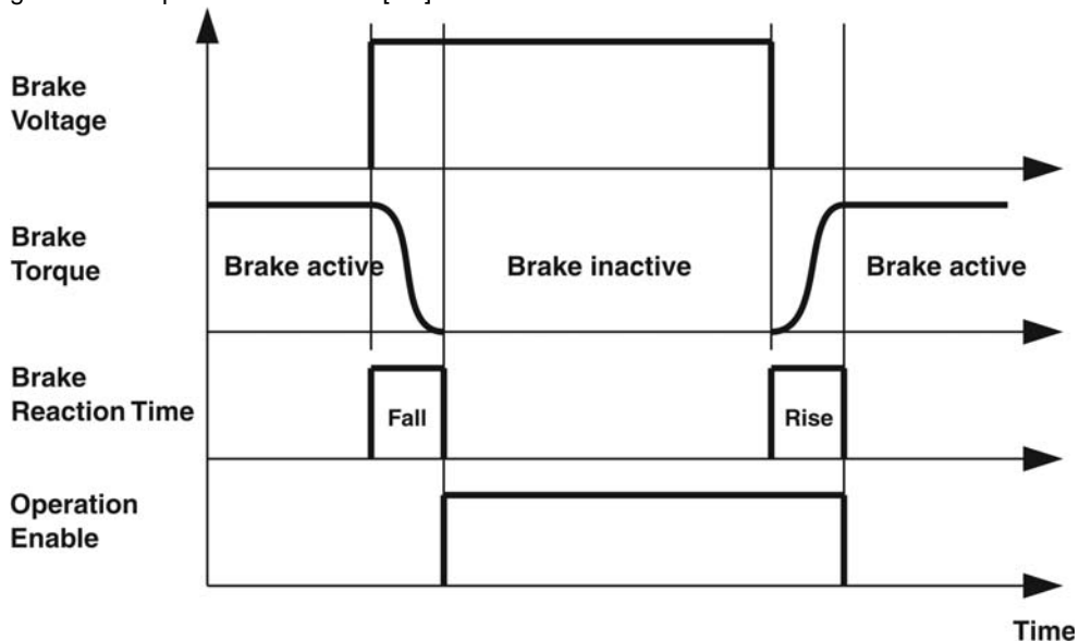
Figure 8-77 Brake Activation Timing
